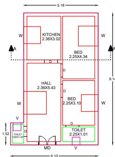
PROPOSED RESIDENTIAL GROUND FLOOR PLAN
