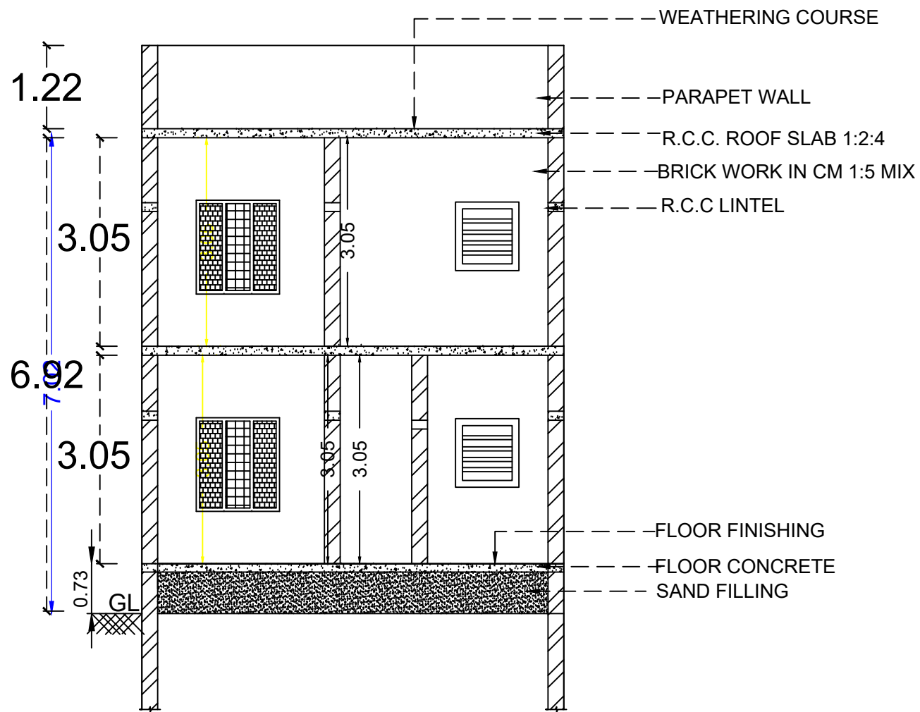
SECTION A1-A1
