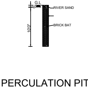
PERCOLATION PIT
