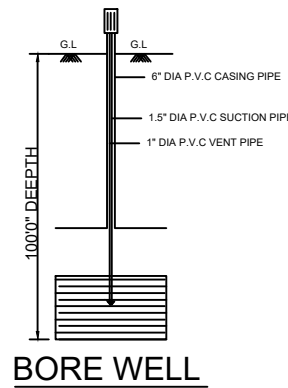
BORE WELL
