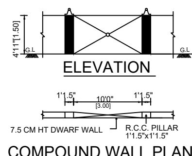
COMPOUND WALL PLAN
