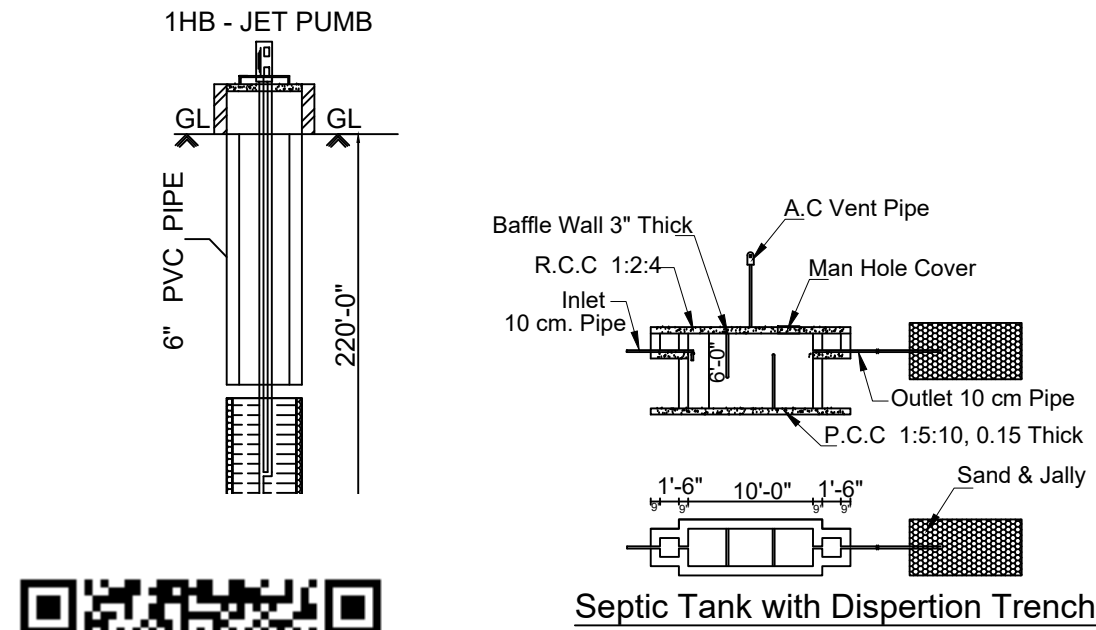
Septic Tank with Dispersion Trench
