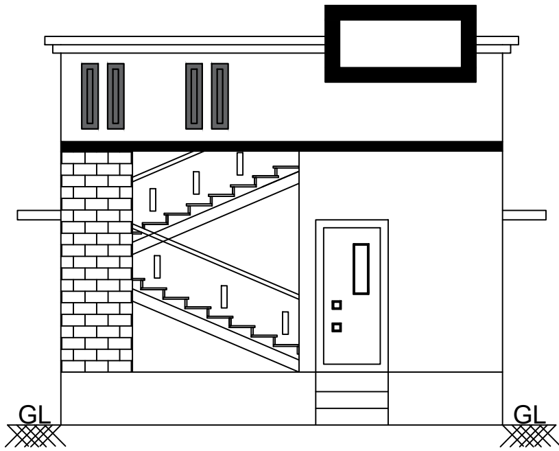
FRONT ELEVATION
