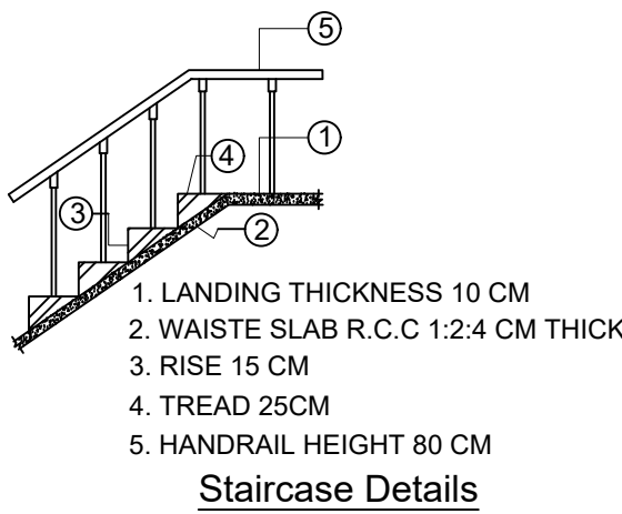
Staircase Details
