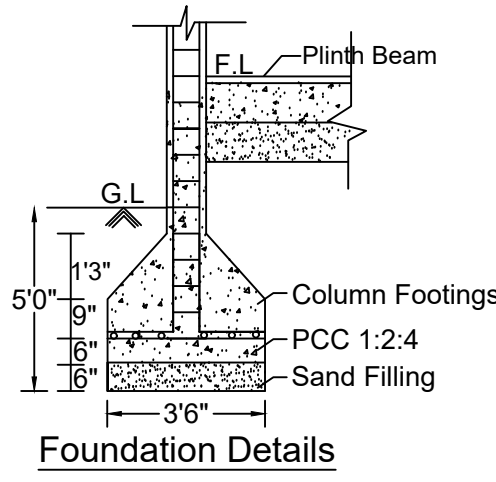
Foundation Details
