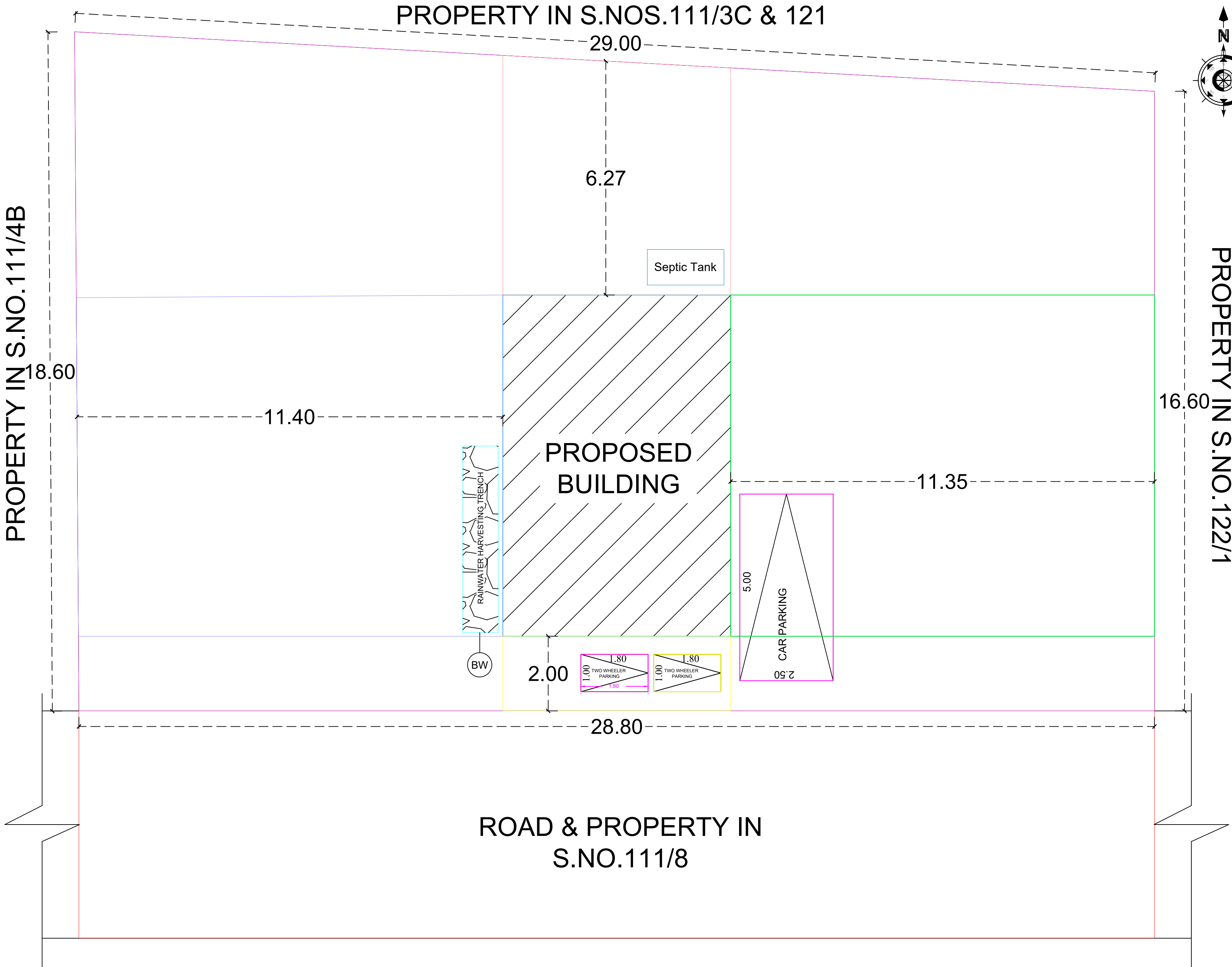
SITE PLAN (1:100)
