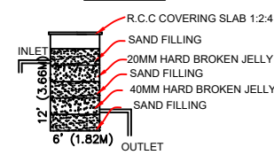
Waste Water Recycle Unit Not To Scale
