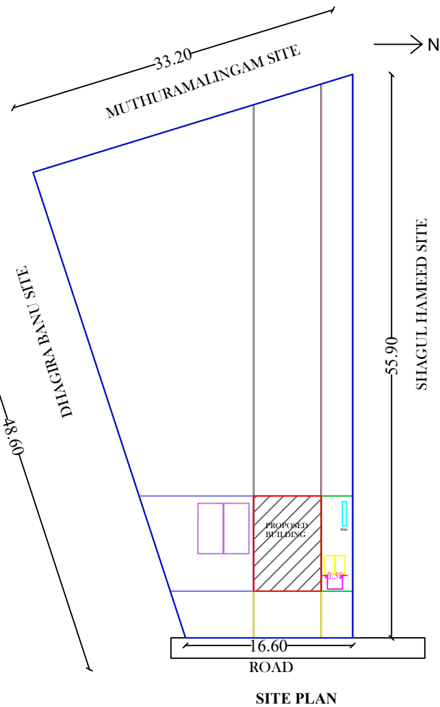
SITE PLAN
