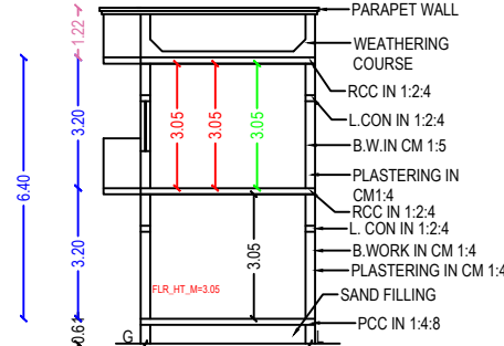
SECTION ON 'RP'
