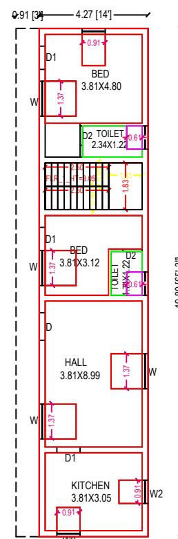
PROPOSED FIRST FLOOR PLAN
