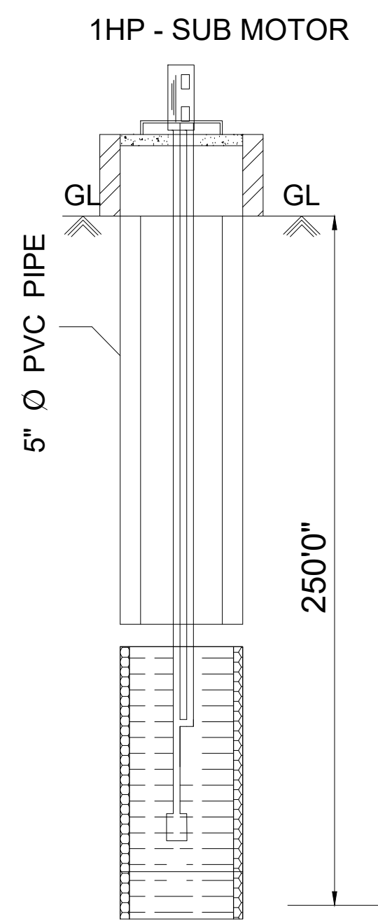
BOREWELL DETAILS
