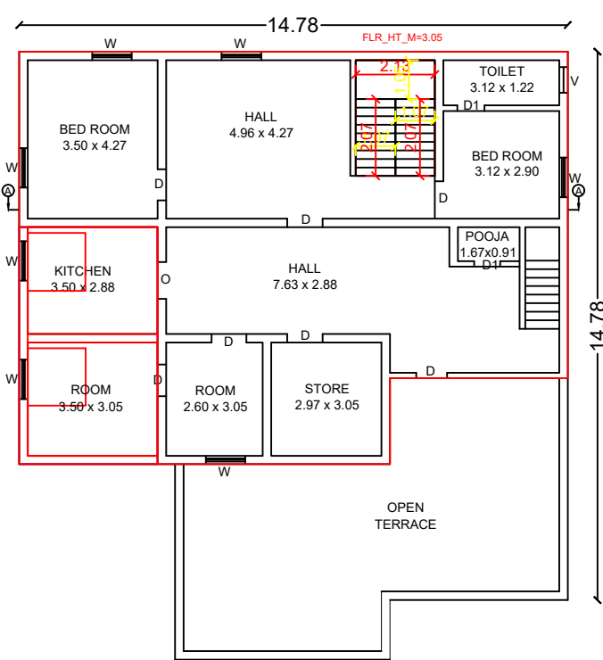
EXI.FIRST FLOOR AND PRO.FIRST FLOOR PLAN
