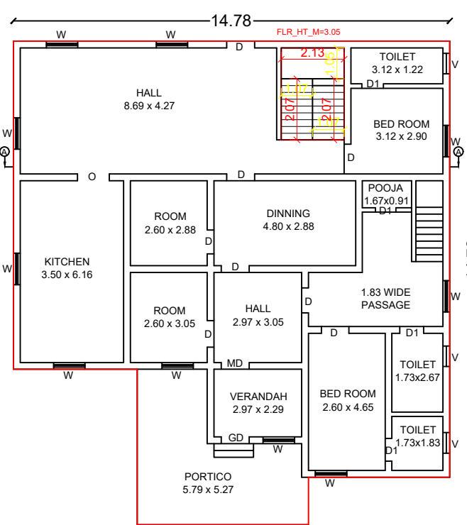
EXI.GROUND FLOOR PLAN
