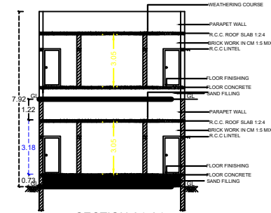
SECTION A1-A1
