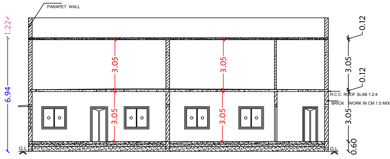
Section on-"AA"
