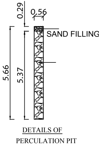
DETAILS OF PERCUSSION PIT
