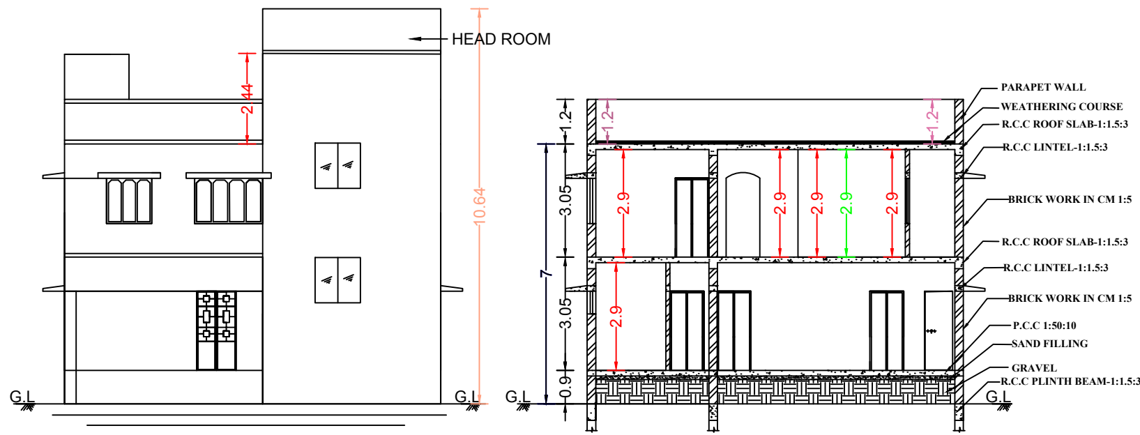
FRONT ELEVATION (SCALE 1:150)
