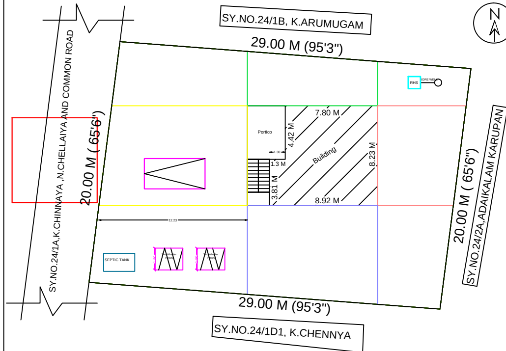
SITE PLAN (1:100)
