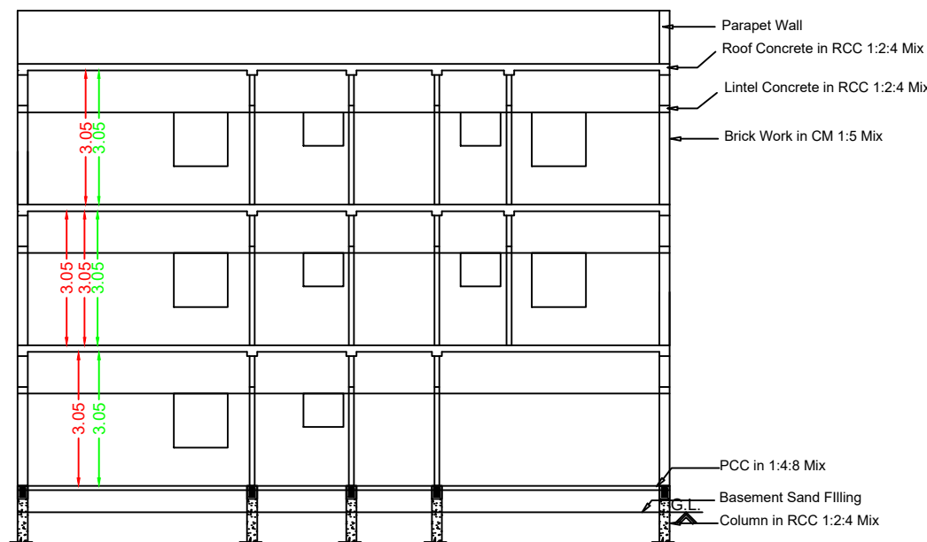
Section RR
