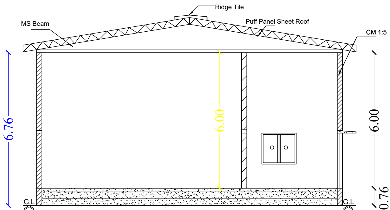
Section on-"AA"
