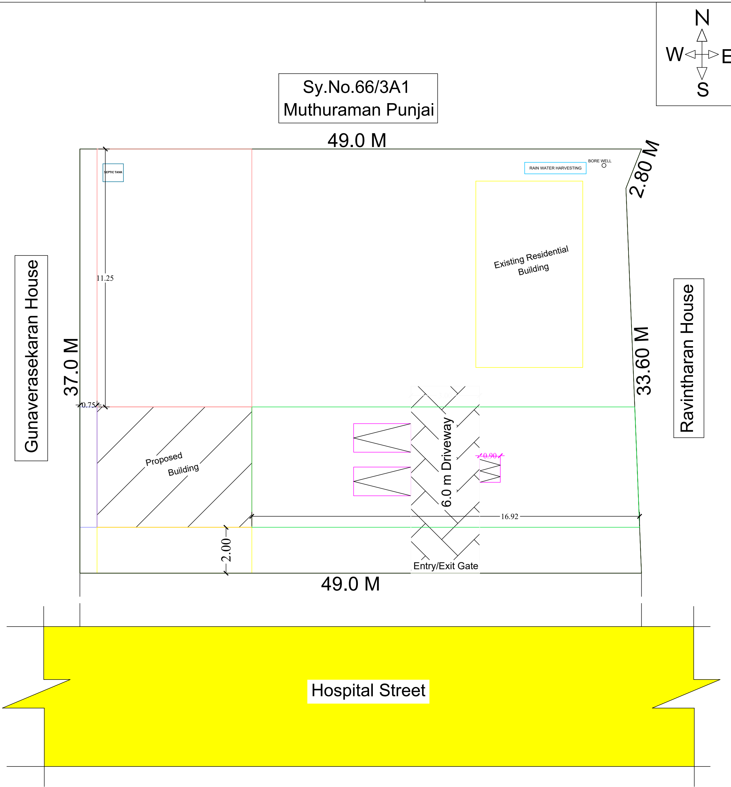
Topo Plan Scale : 1:100
