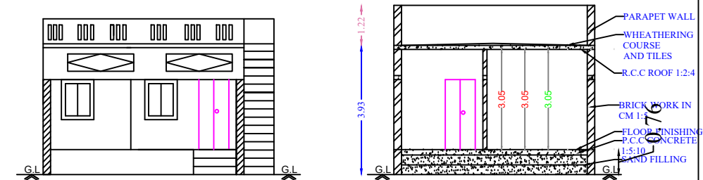
Section on-"AA"
