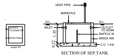
SECTION OF SEP.TANK
