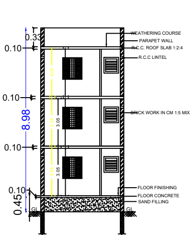
SECTION A1-A1
