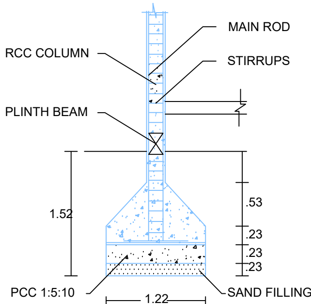
COLUMN DETAILS
