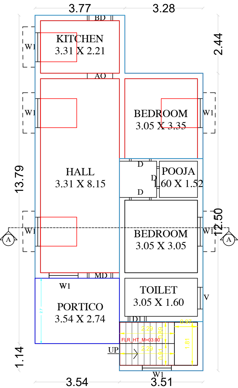
PRO. ADDITIONAL GROUND FLOOR PLAN
