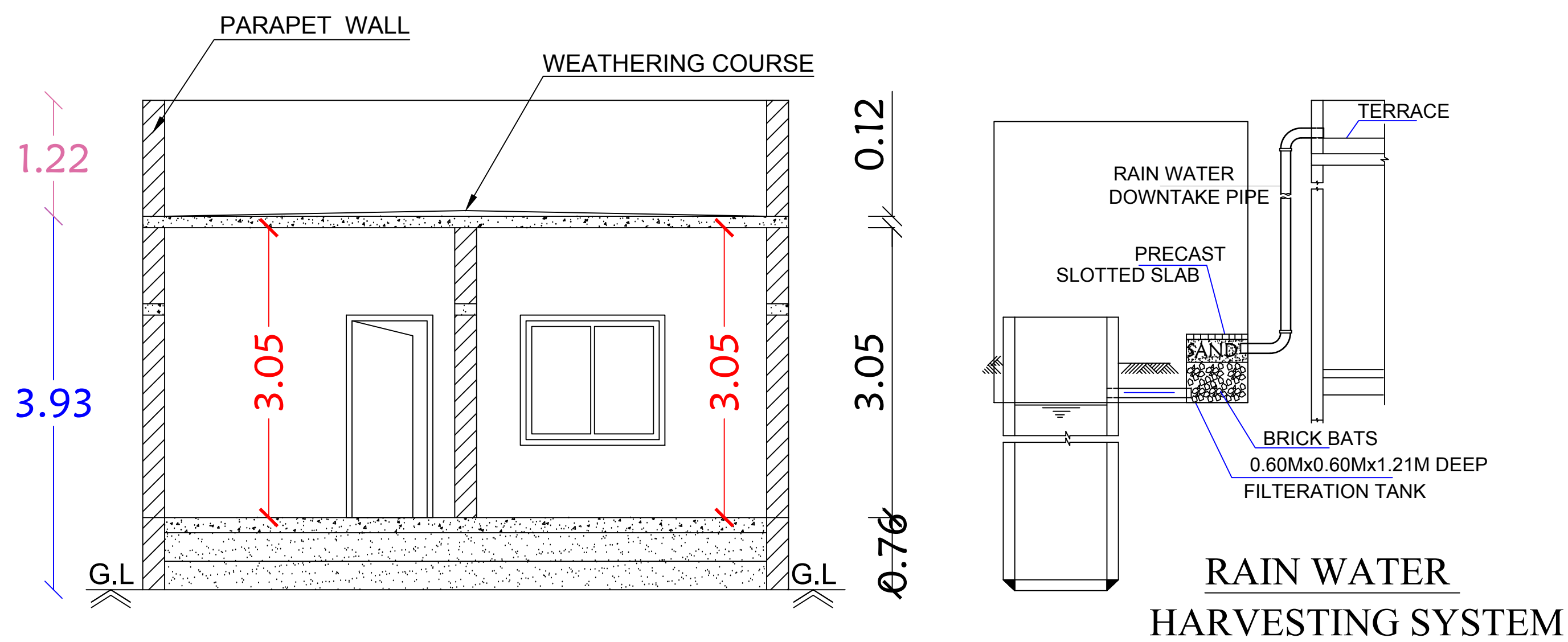
Section on-"AA"
