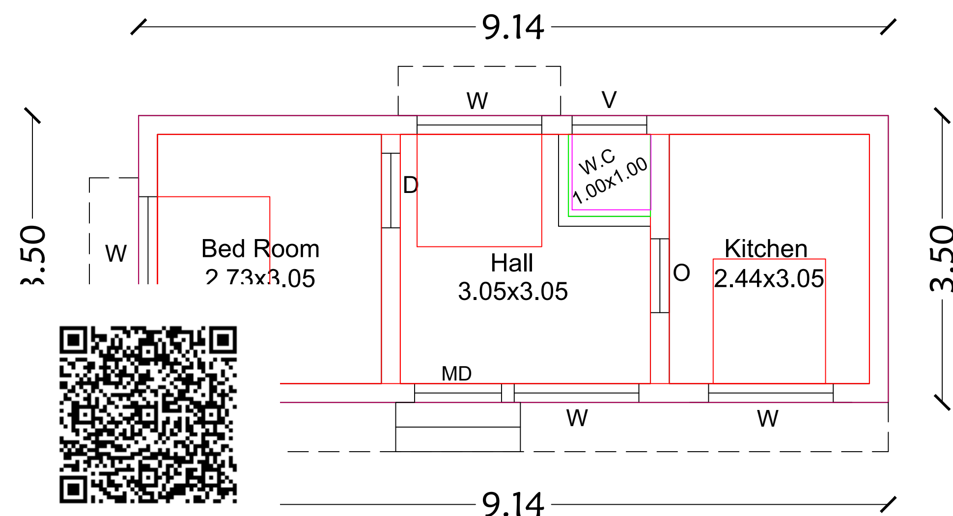
Ground Floor
