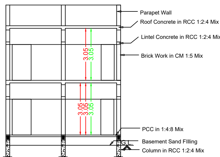
Section RR
