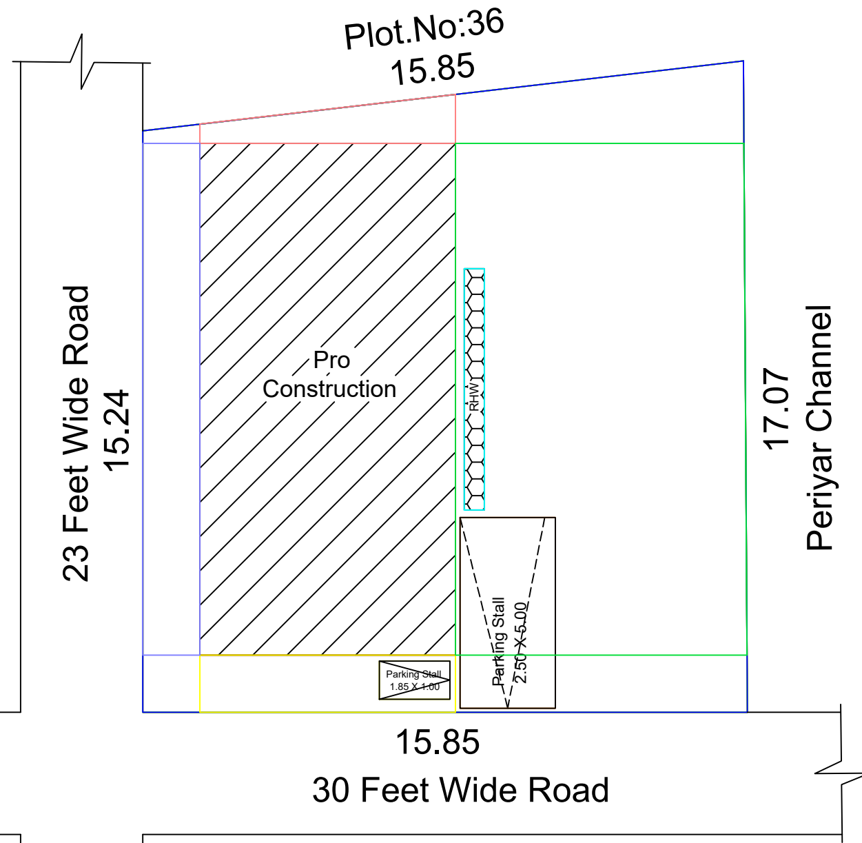
SITE PLAN
