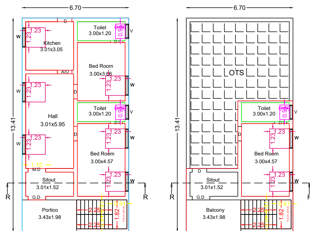
Pro.Ground & First Floor Plan
