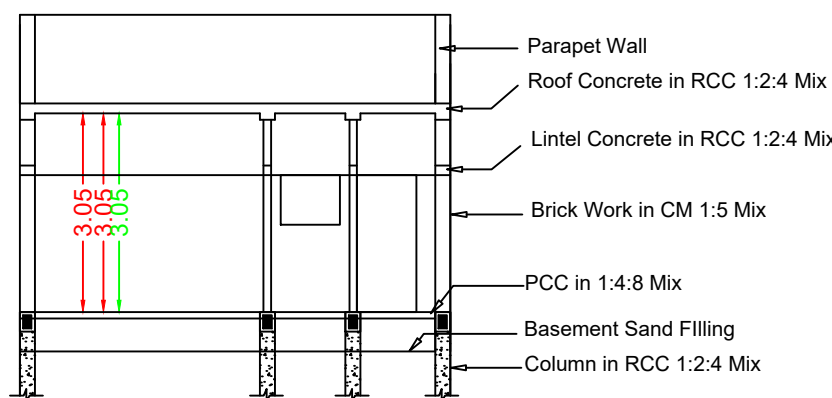
Section RR
