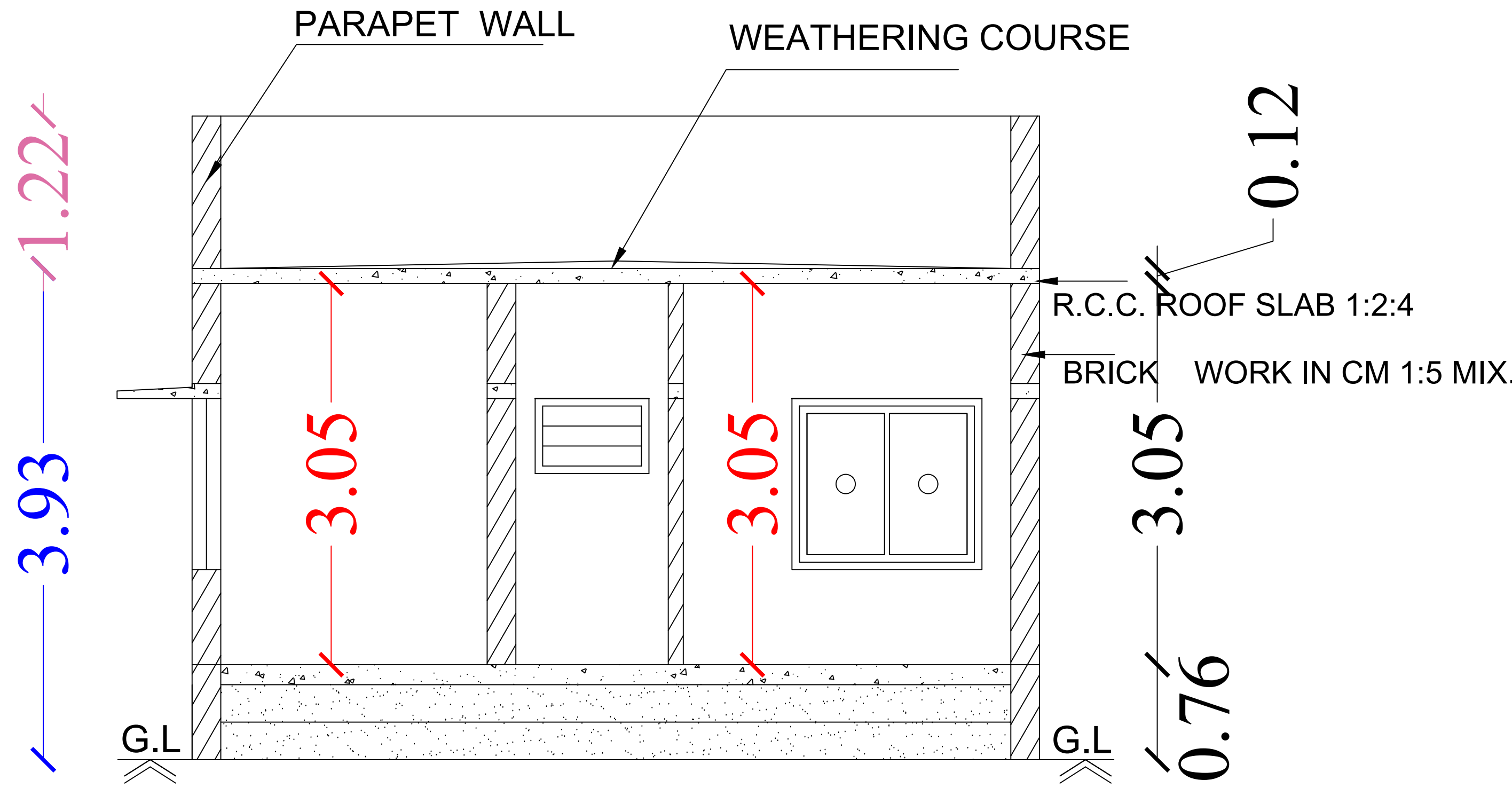
Section on-"AA"
