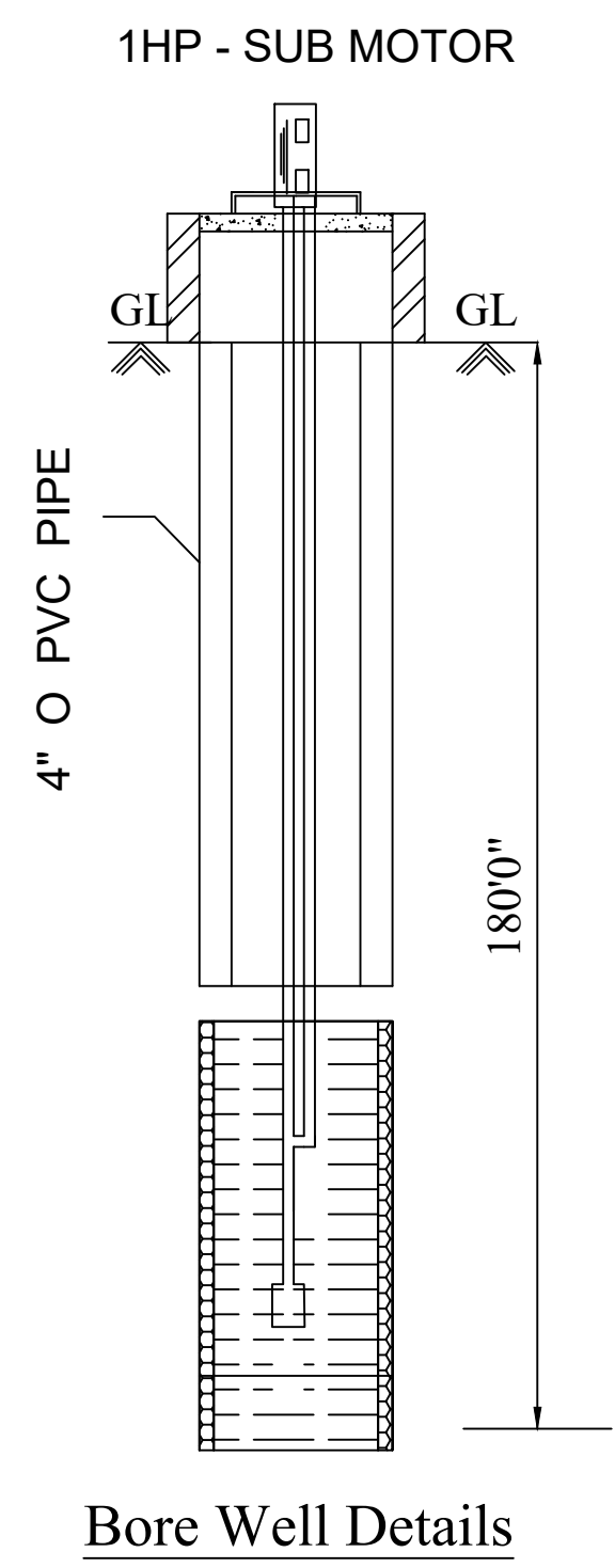
Bore Well Details
