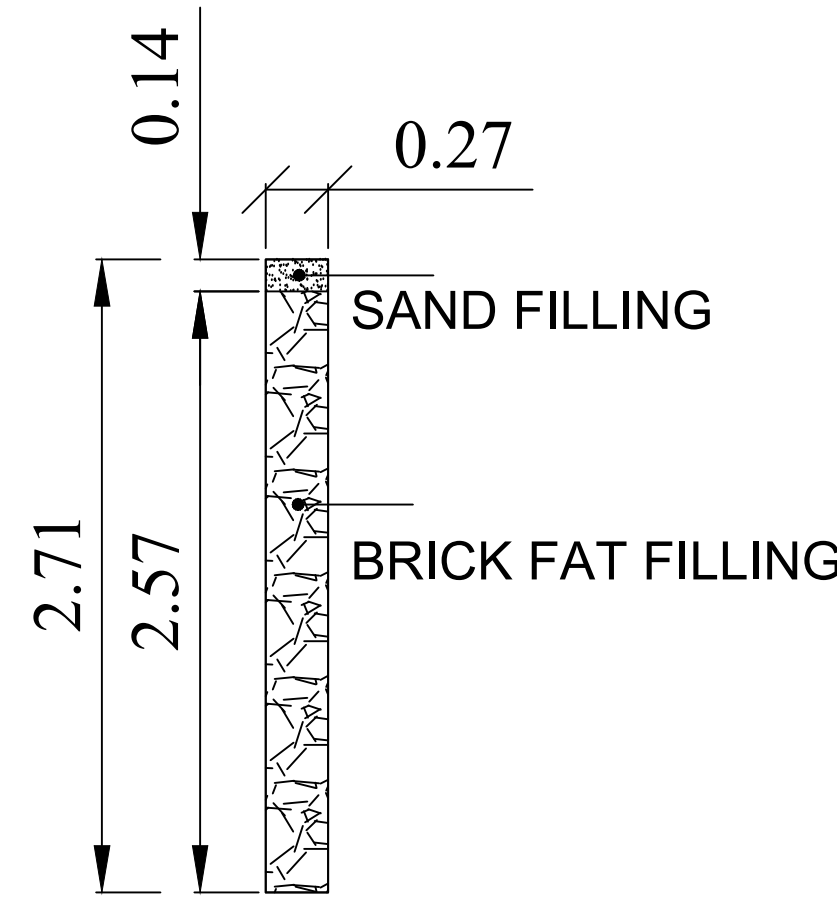
DETAILS OF PERCULATION PIT
