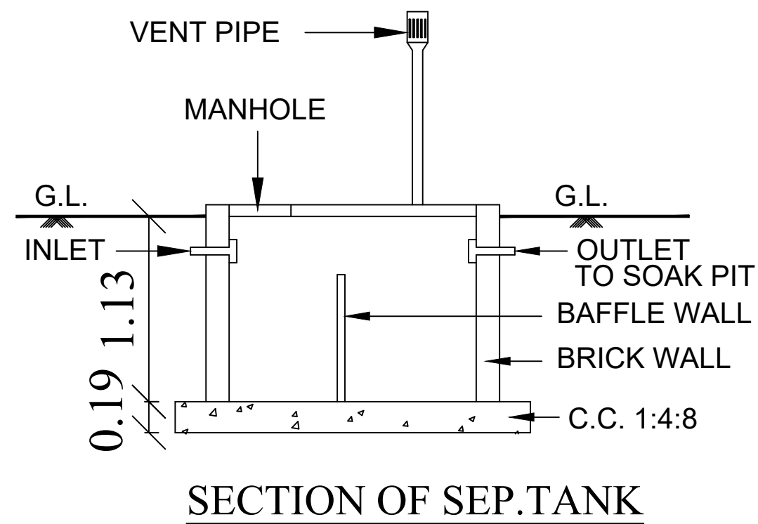
SECTION OF SEP. TANK
