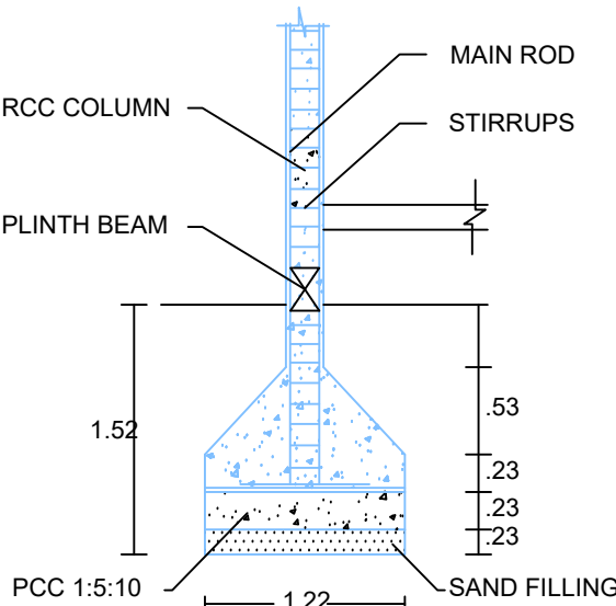
COLUMN DETAILS
