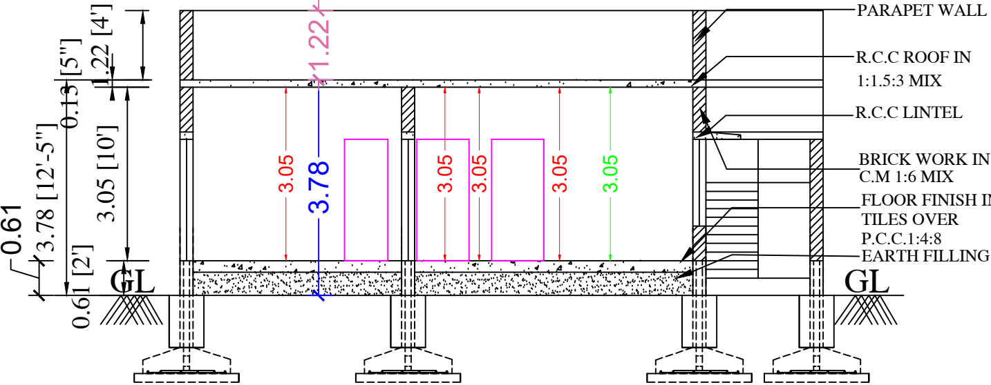
SECTION AA
