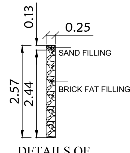
DETAILS OF PERCOLATION PIT
