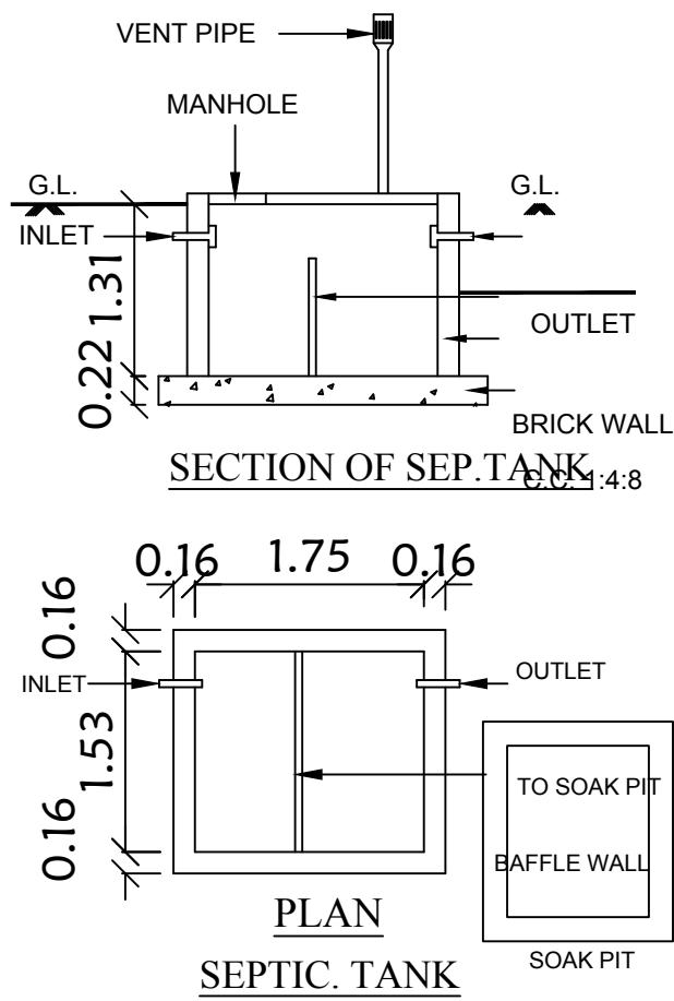
SECTION OF SEP. TANK
