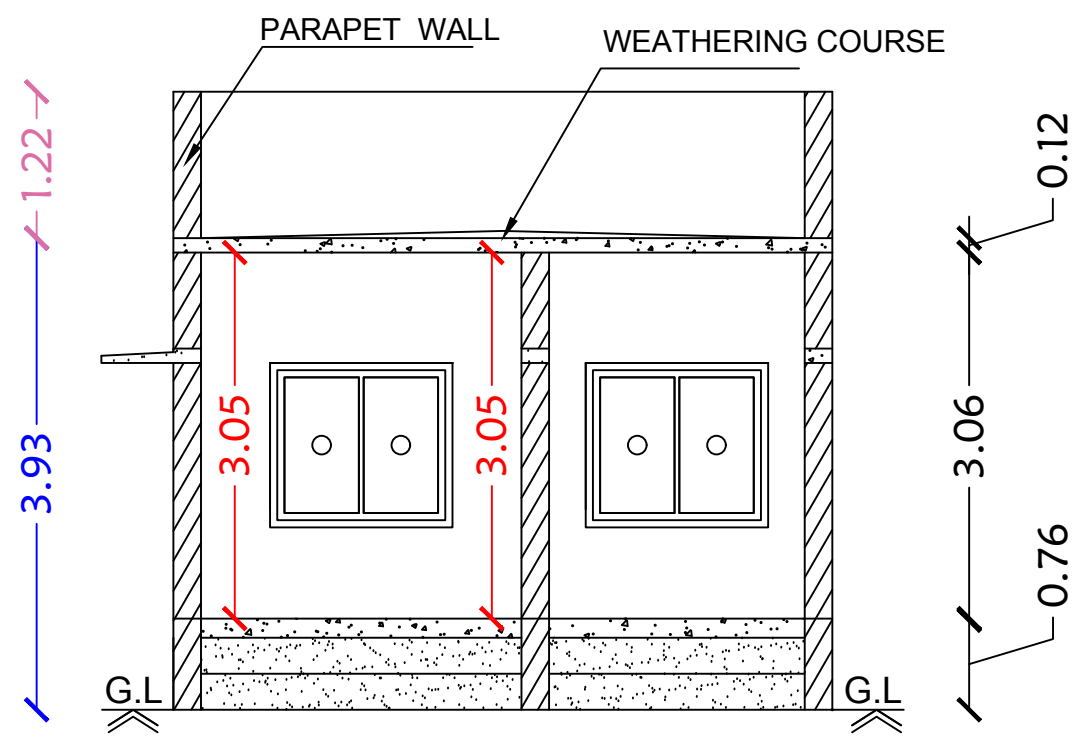
Section on-"AA"
