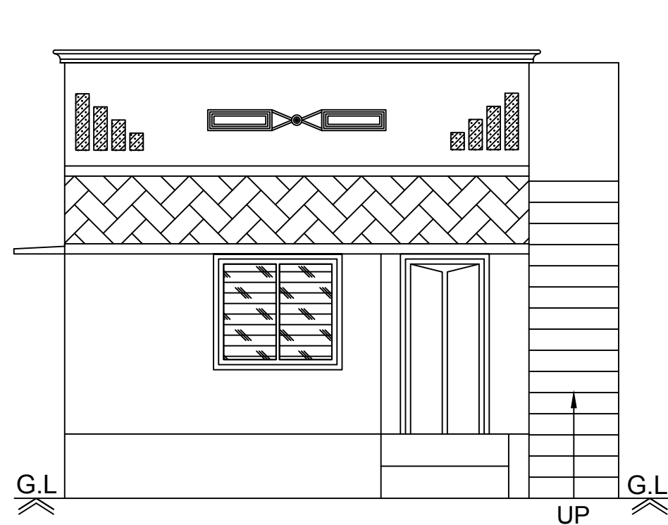
Front Elevation
