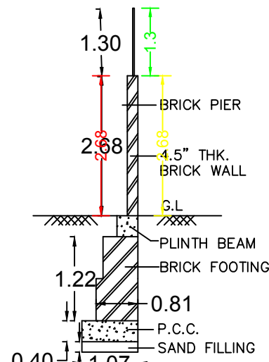
COMPOUND WALL DETAILS
