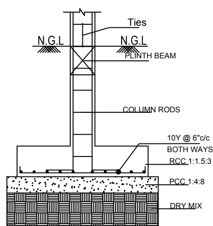
FOUNDATION DETAILS (Concentric Footing)
