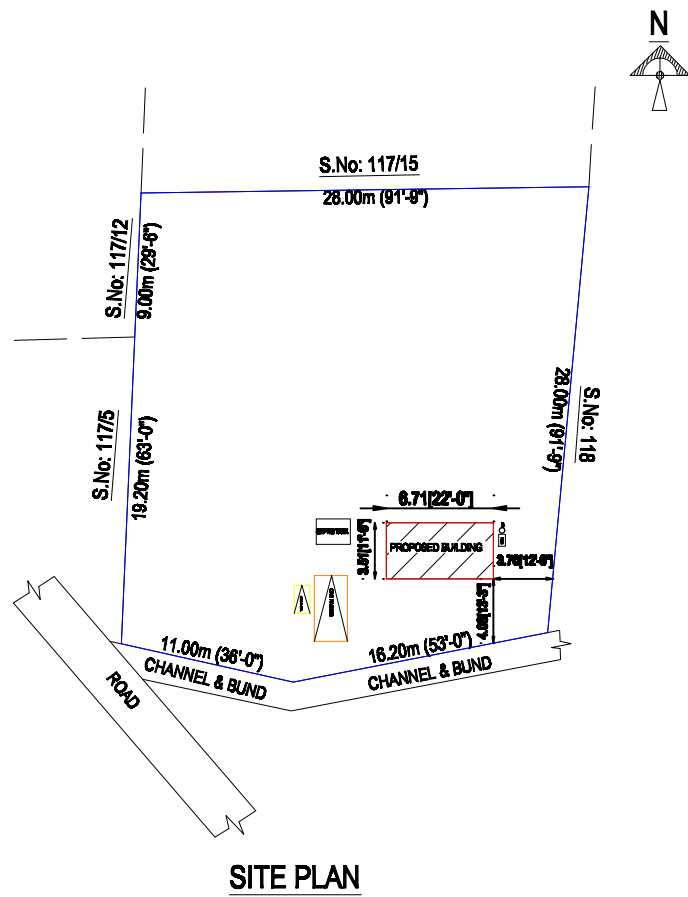
SITE PLAN
