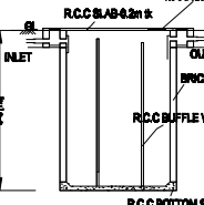
SECTION- SEPTIC TANK
