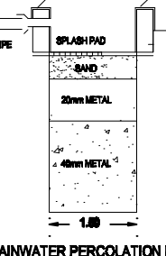
RAINWATER PERCOLATION PIT
