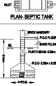
FOUNDATION DETAILS
