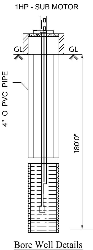
Bore Well Details
