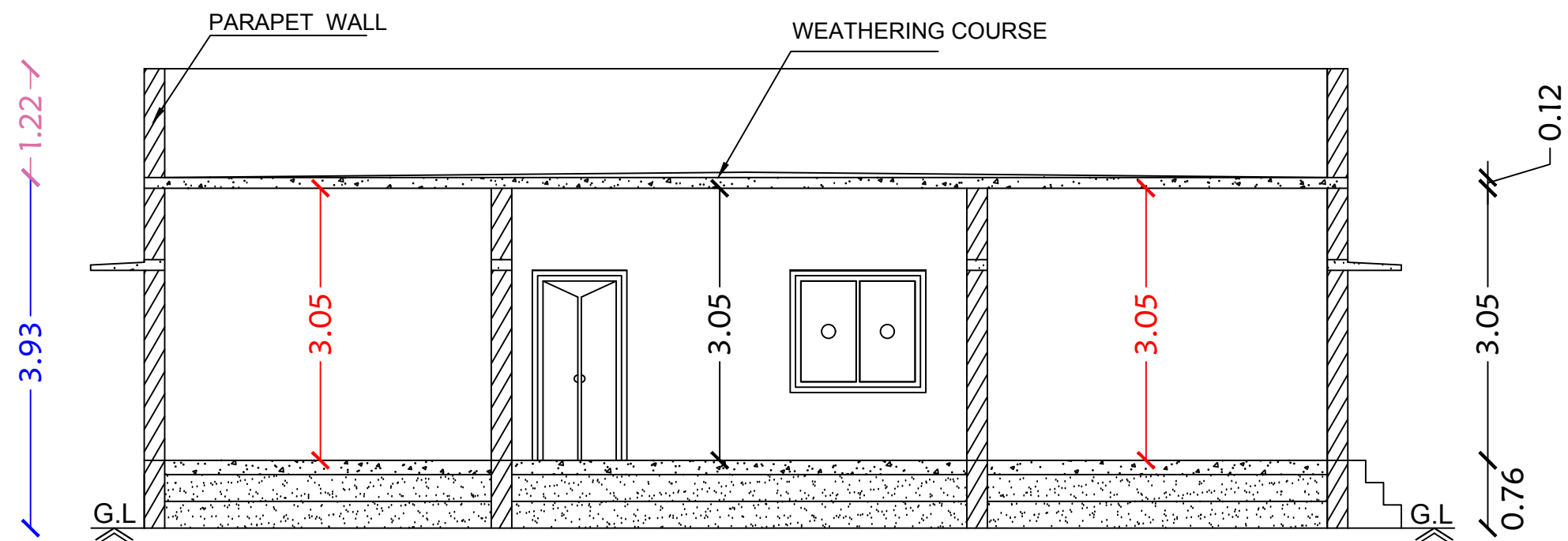
Section on-"AA"
