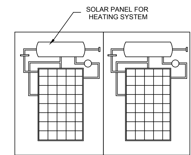
SOLAR HEATING SYSYTEM
