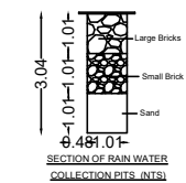
SECTION OF RAIN WATER COLLECTION PITS (NTS)
