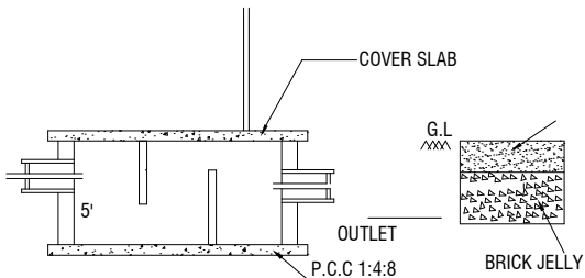
SECTION-AB
