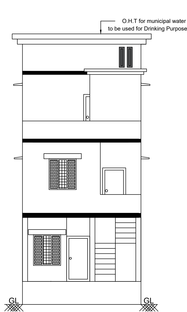
FRONT ELEVATION
