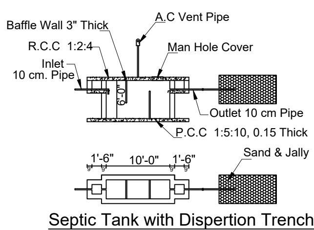
Septic Tank with Dispersion Trench
