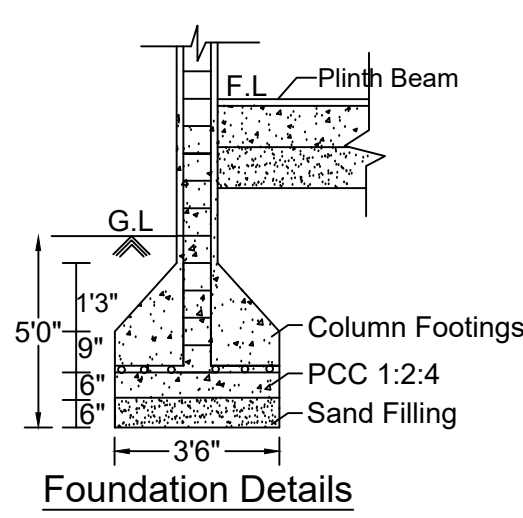
Foundation Details
