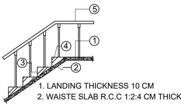
Staircase Details
