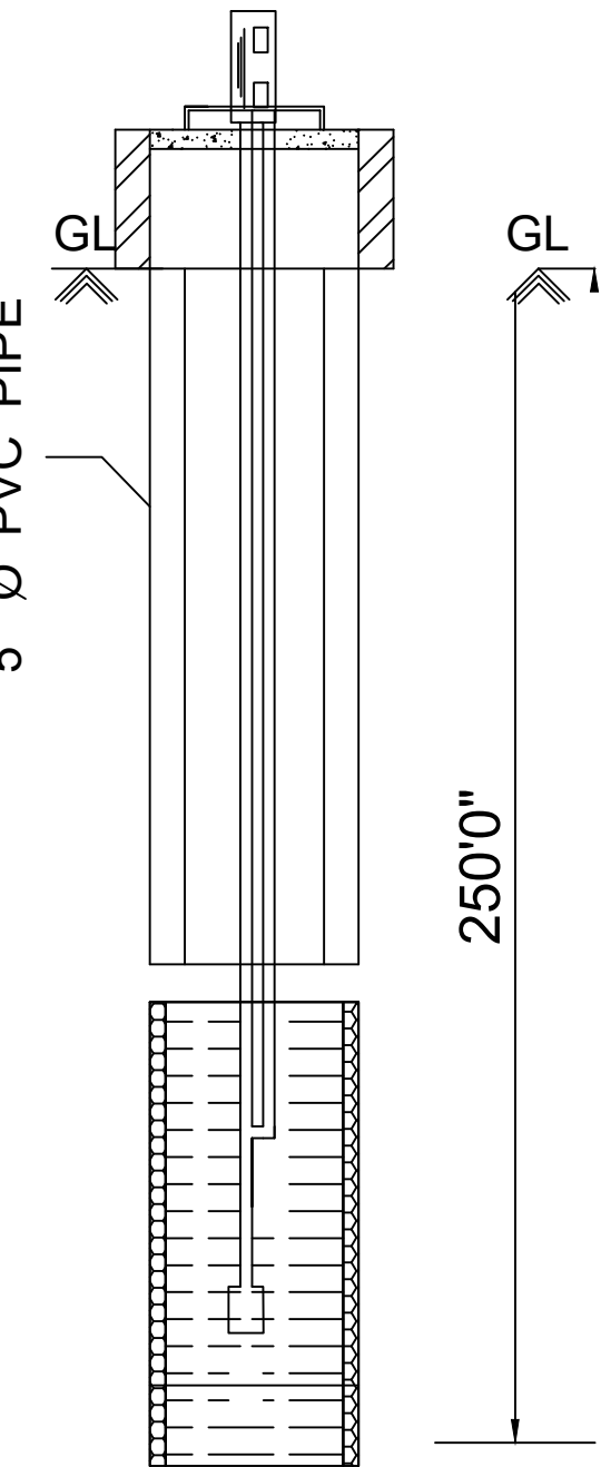
BOREWELL DETAILS
