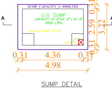
SUMP DETAIL
