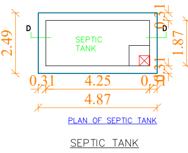
SEPTIC TANK
