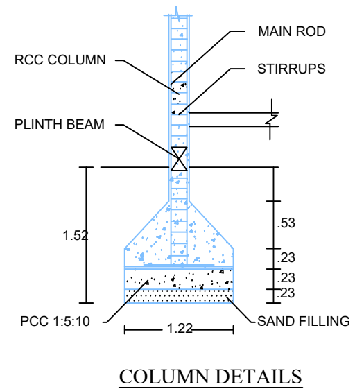
COLUMN DETAILS
