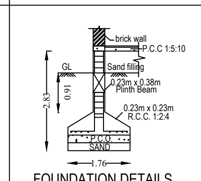
FOUNDATION DETAILS
