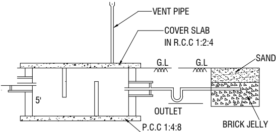
DETAILS OF RAIN WATER HARVESTING STRUCTURES
