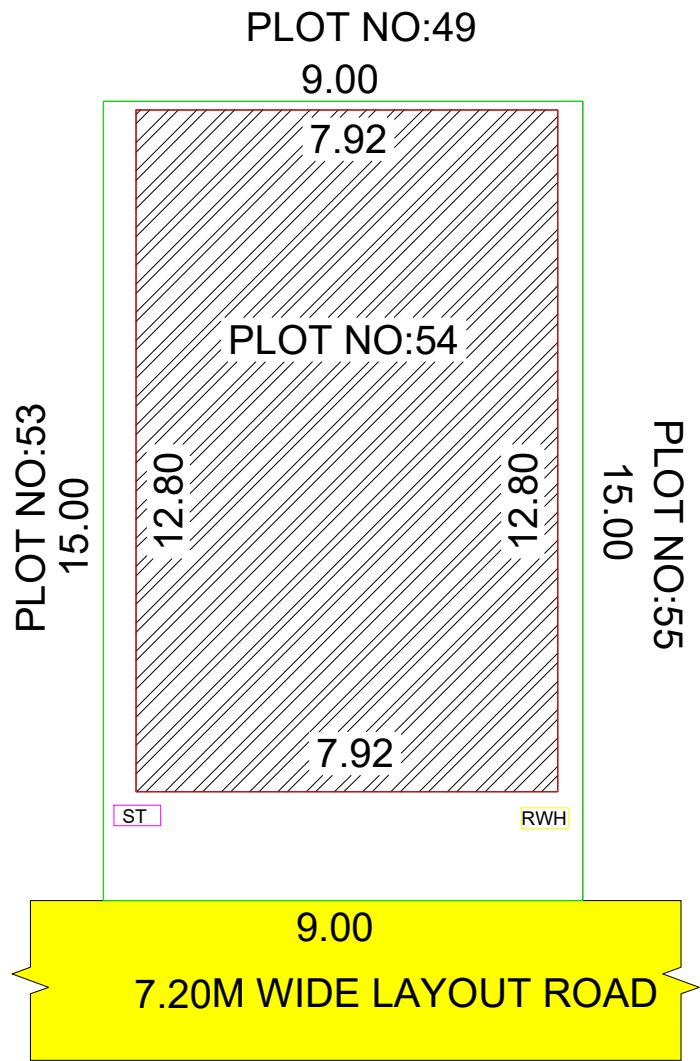
SITE PLAN
