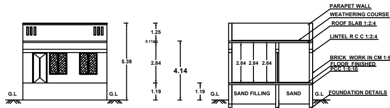
FRONT ELEVATION
