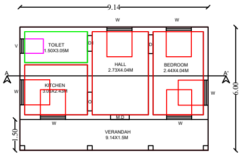
PROPOSED GROUND FLOOR
