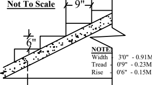
Staircase Detail
