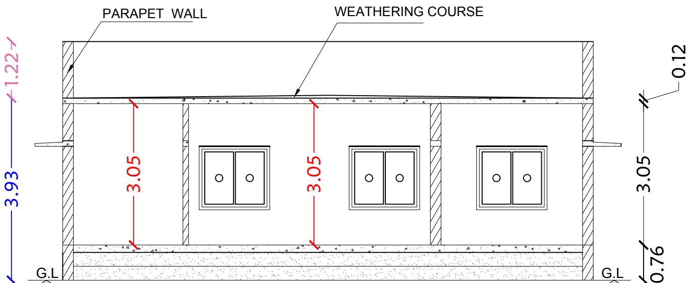
Section on-"AA"
