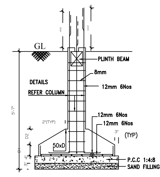
FOUNDATION DETAILS
