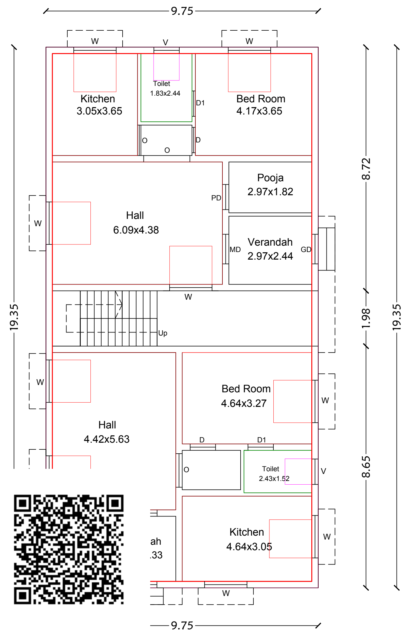
Ground Floor
