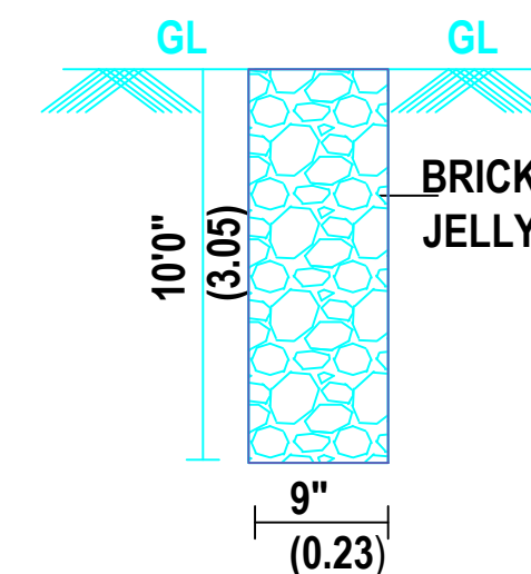
PERCOLATION PIT
