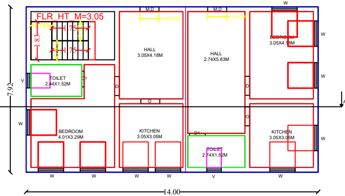
PROPOSED FIRST FLOOR
