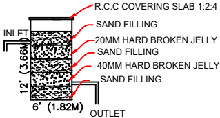
Waste Water Recycle Unit Not To Scale
