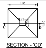
FOUNDATION DETAILS
