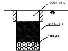
IN WATER HARVESTING SYSTEM (NOT TO SCALE)
