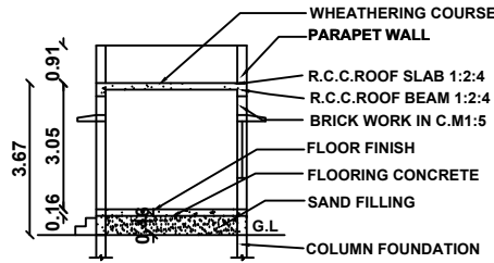
SECTION ON GG
