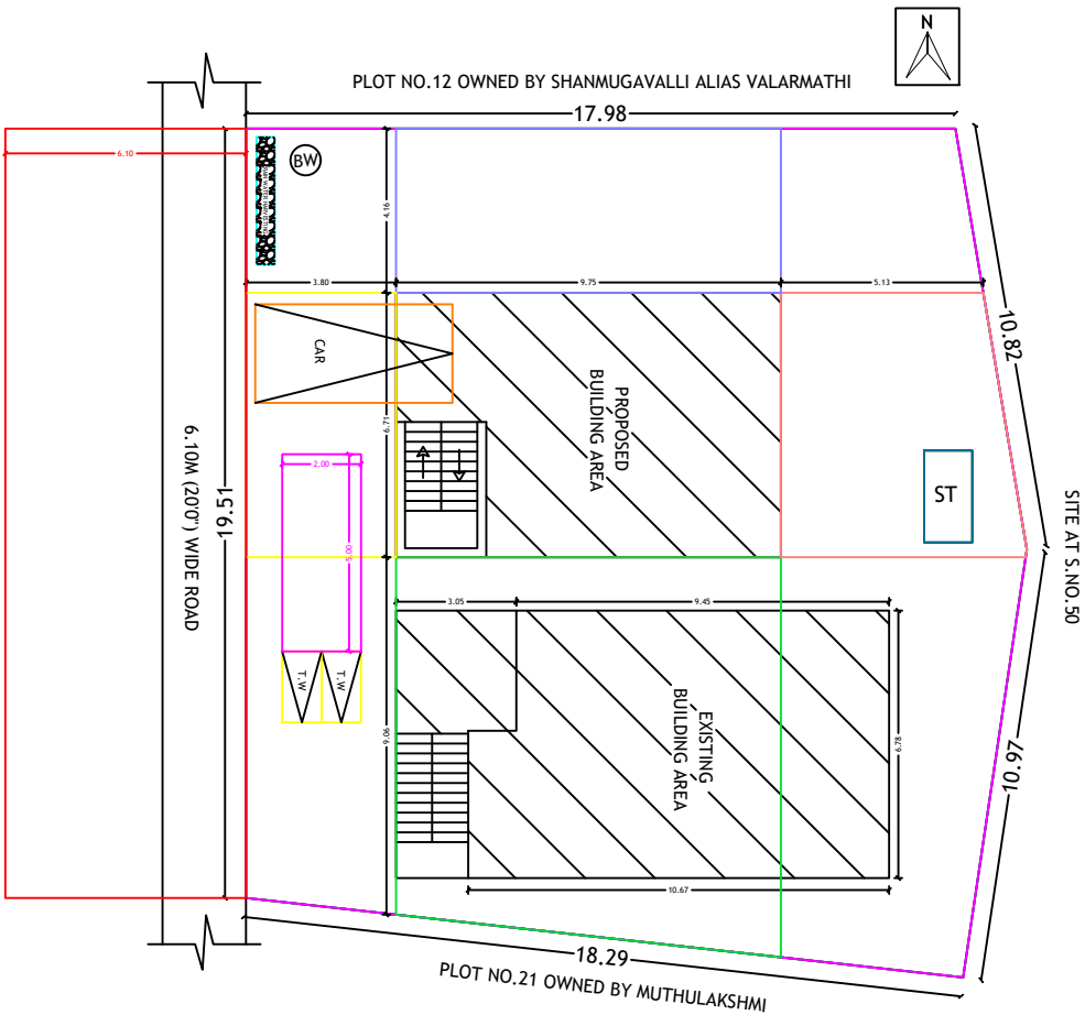
SITE PLAN
