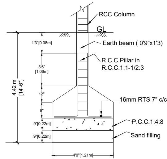
FOUNDATION DETAILS
