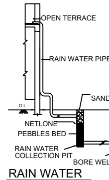
RAIN WATER HARVESTING SYSTEM
