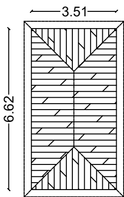
TERRACE PLAN
