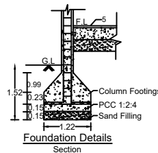
Foundation Details
