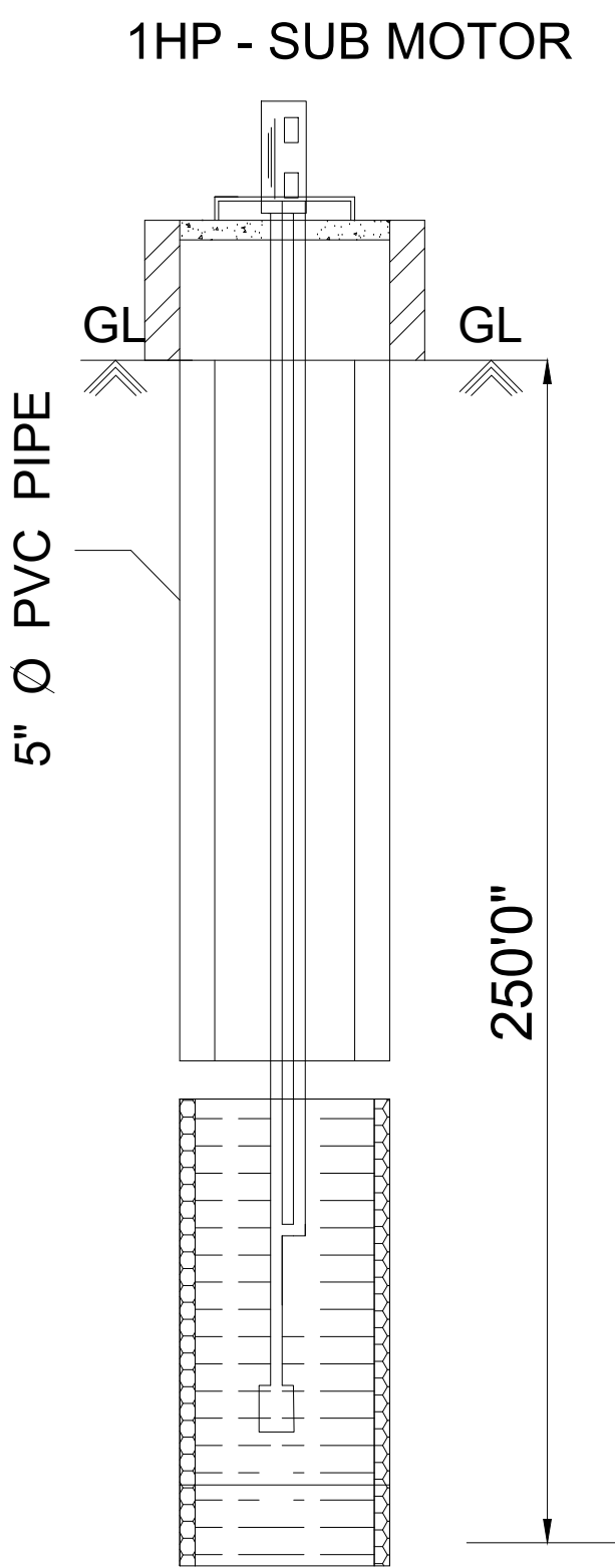
BOREWELL DETAILS
