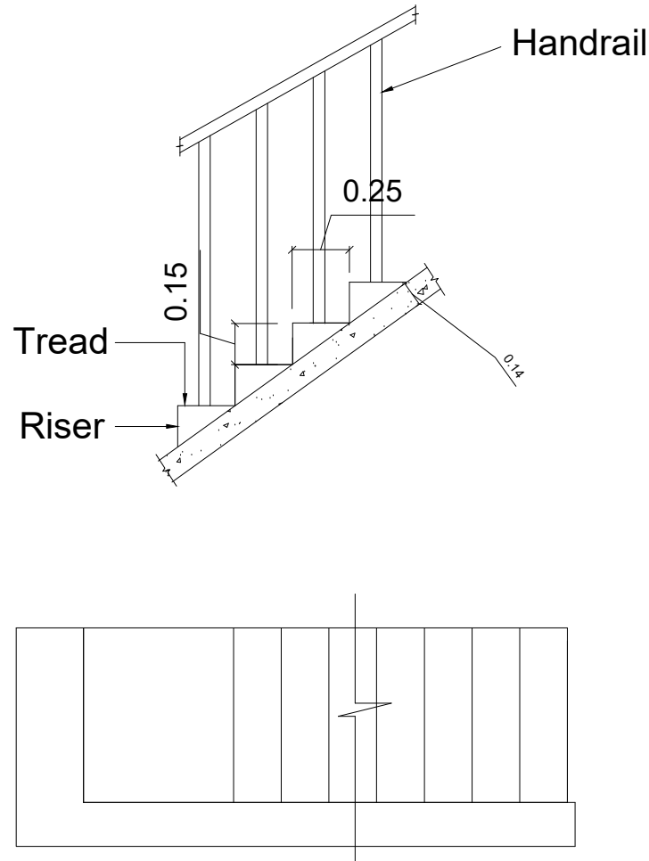
STAIRCASE DETAIL
