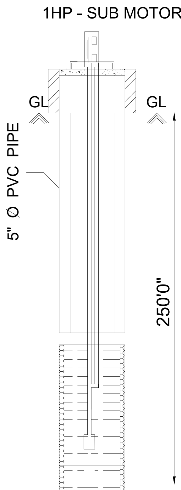
BOREWELL DETAILS
