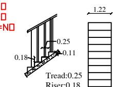
STAIRCASE DETAIL
