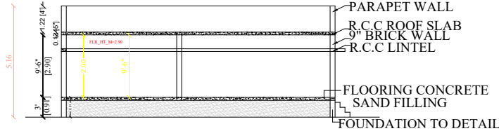
SECTION ON 'AA'
