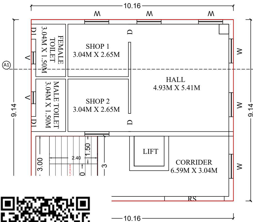
OUND FLOOR PLAN
