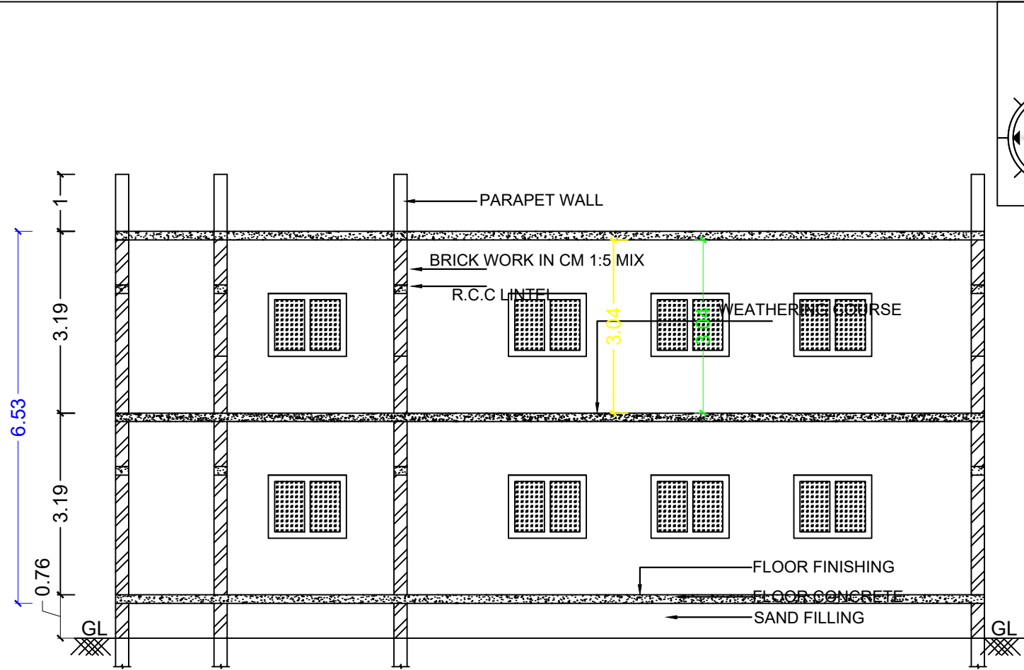
SECTION AT A1-A1
