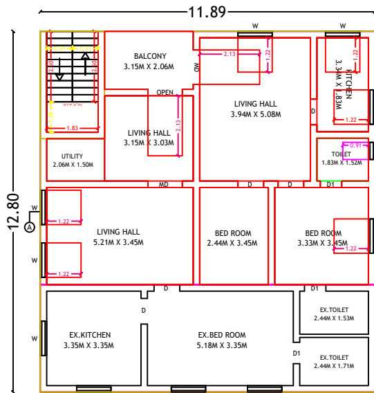
EXISTING & PROPOSED FIRST FLOOR PLAN
