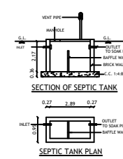
SEPTIC TANK PLAN
