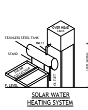
SOLAR WATER HEATING SYSTEM
