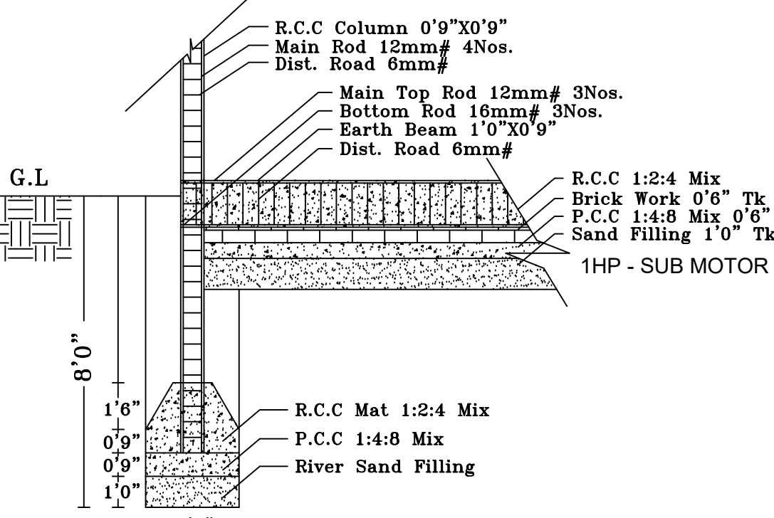
FOUNDATION DETAILS
