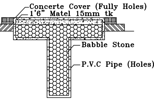
RAIN WATER STOREAGE TANK
